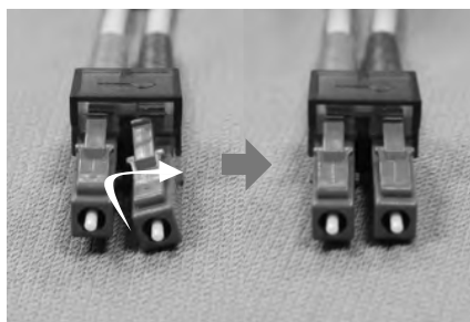
Rotate the LC Connector until it clicks into place
