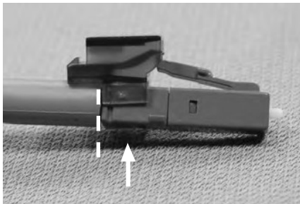
Place the LC Connector into one half of the LC Lock
