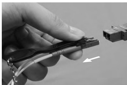
Holding Connector & Key together pull them out
