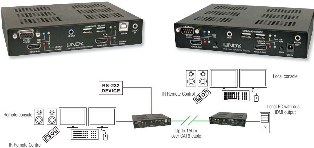
150m CAT6 KVM Extender with Dual Head HDMI, USB, Audio, IR & RS-232
