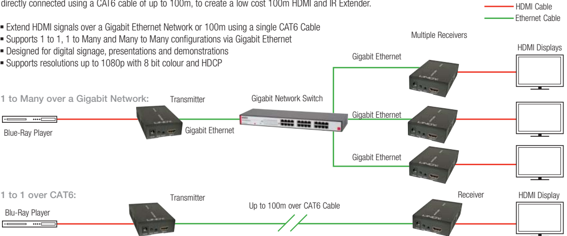
100m HDMI over Gigabit Ethernet IP Extender
