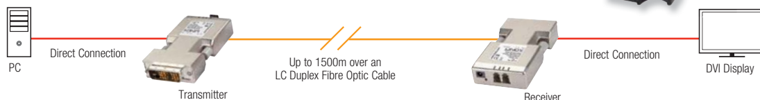
1500m Fibre Optic DVI-D Single Link Extender
