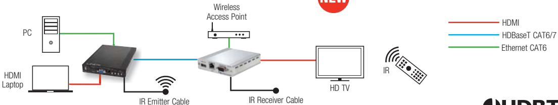
HDBaseT C6 HDMI/VGA Switching Extender Transmitter, 100m 38215 C6 HDMI Receiver Premium with HDBaseT, 100m 38218
