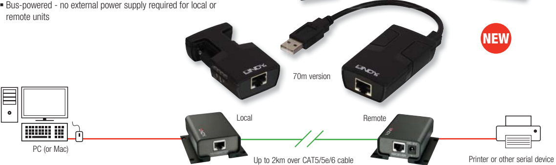
70m CAT5 USB to RS-232 Serial Extender
