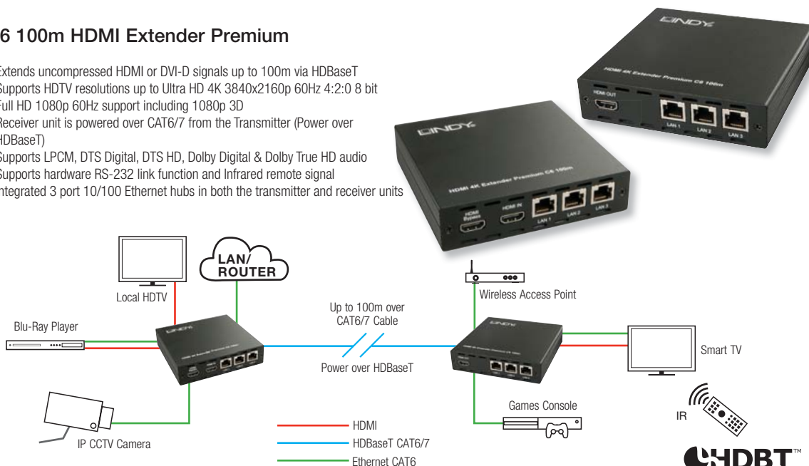
C6 100m HDMI Extender Premium
