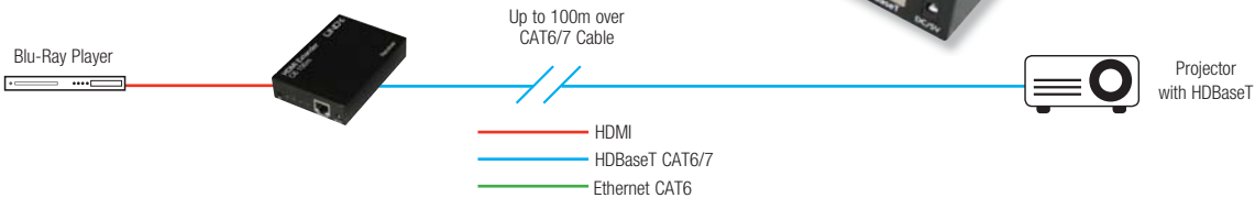
C6 HDMI 100m Transmitter with HDBaseT 38019
