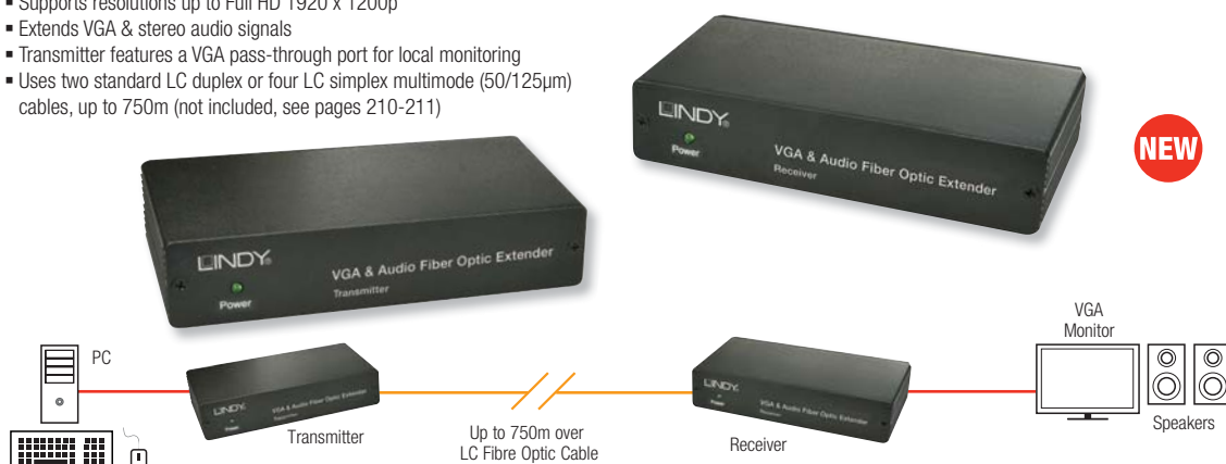
750m VGA & Audio Fibre Optic Extender
