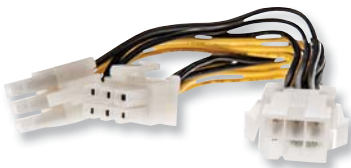
6 Way PCIe Female to 2 x 6 Way PCIe Male
