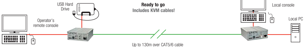
130m CAT6 DVI-D & USB KVM Extender for Mass Storage
