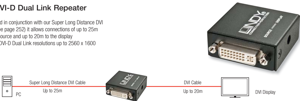
45m DVI-D Dual Link Repeater
