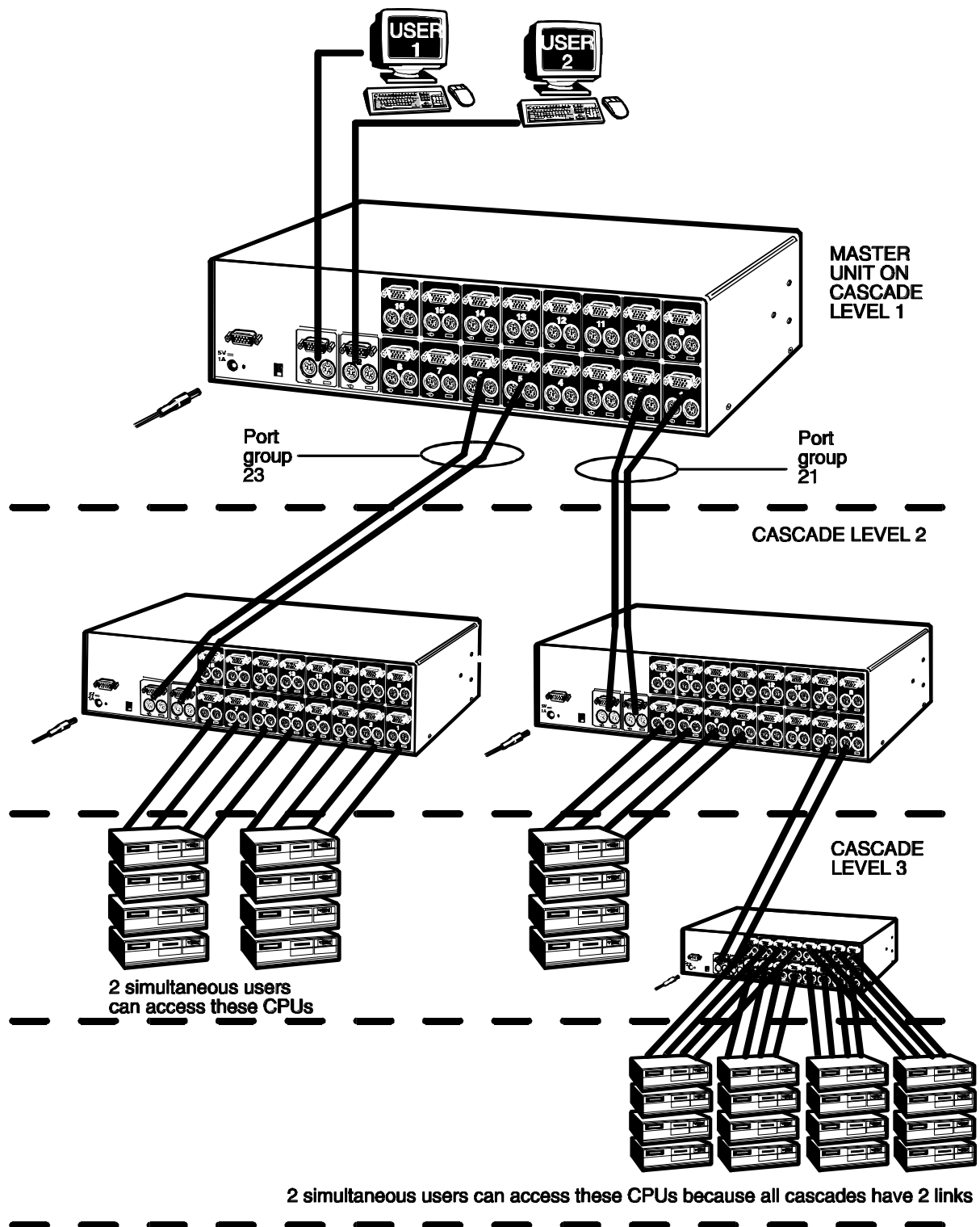
Fig. 4 - A cascaded application using multiple LINDY CPU Switch Dual Junior units
