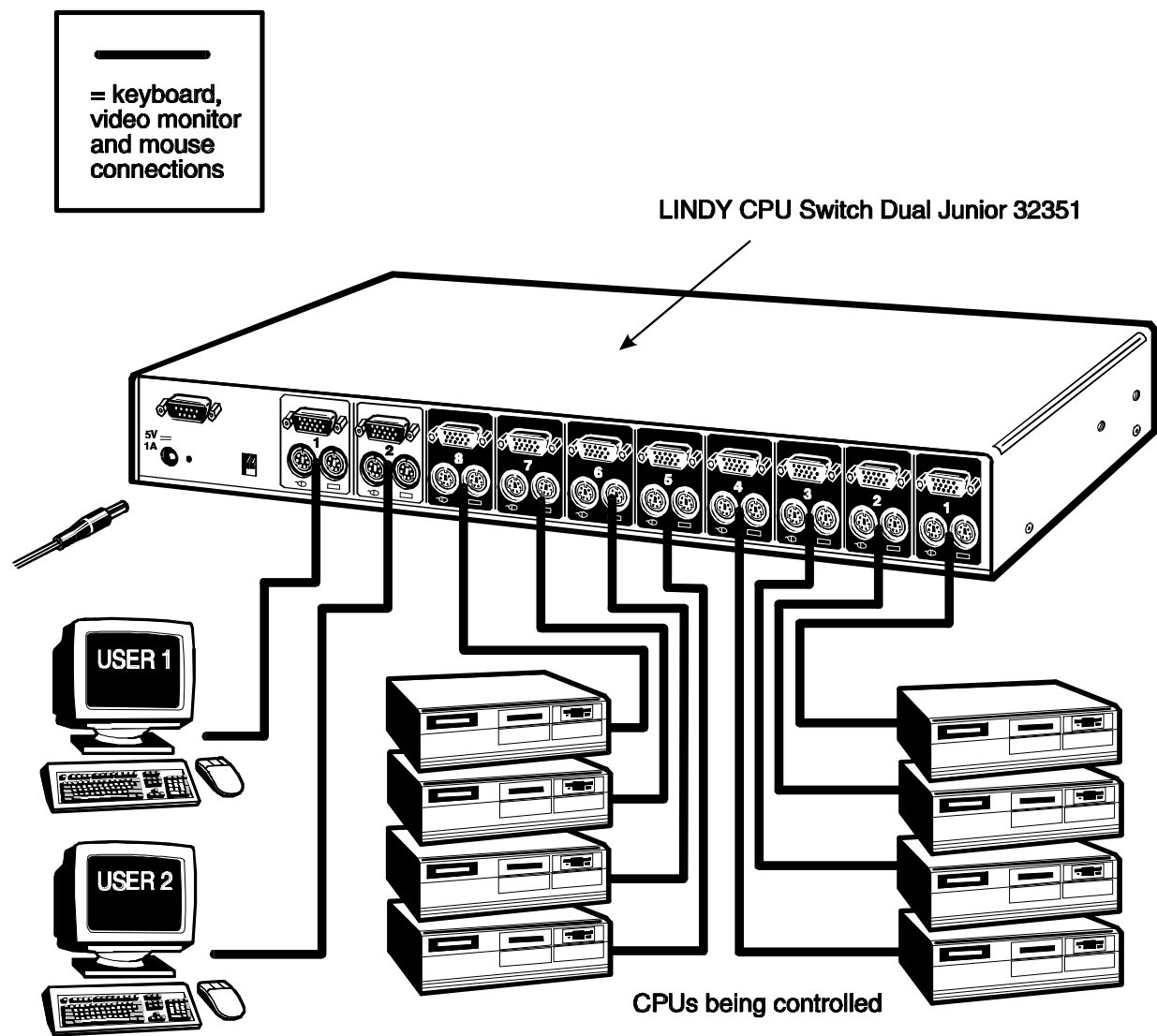
Fig. 3 - A typical installation using a single LINDY CPU Switch Dual Junior 32351
